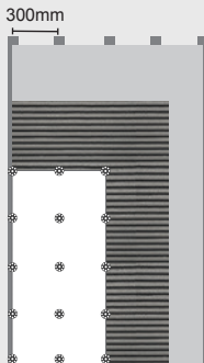
Indicative Fixing Detail using adhesive, washers & screws based on 300mm stud centres (1200mm x 600mm x 12.5mm VipaBoard)
