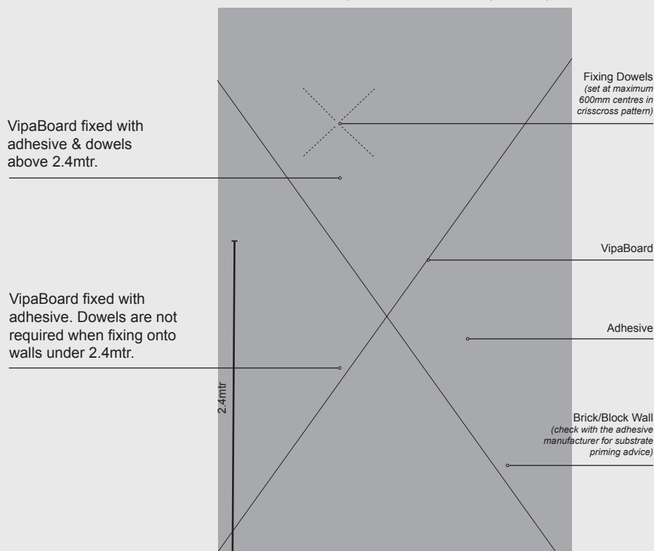
Indicative Fixing Detail using adhesive and fixing dowels. (1200mm x 600mm VipaBoard)
