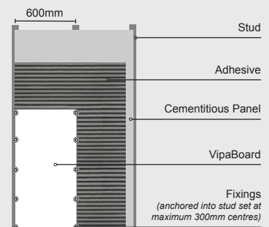
Indicative Fixing Detail using adhesive, washers & screws based on 600mm stud centres (1200mm x 600mm x 20mm VipaBoard)
